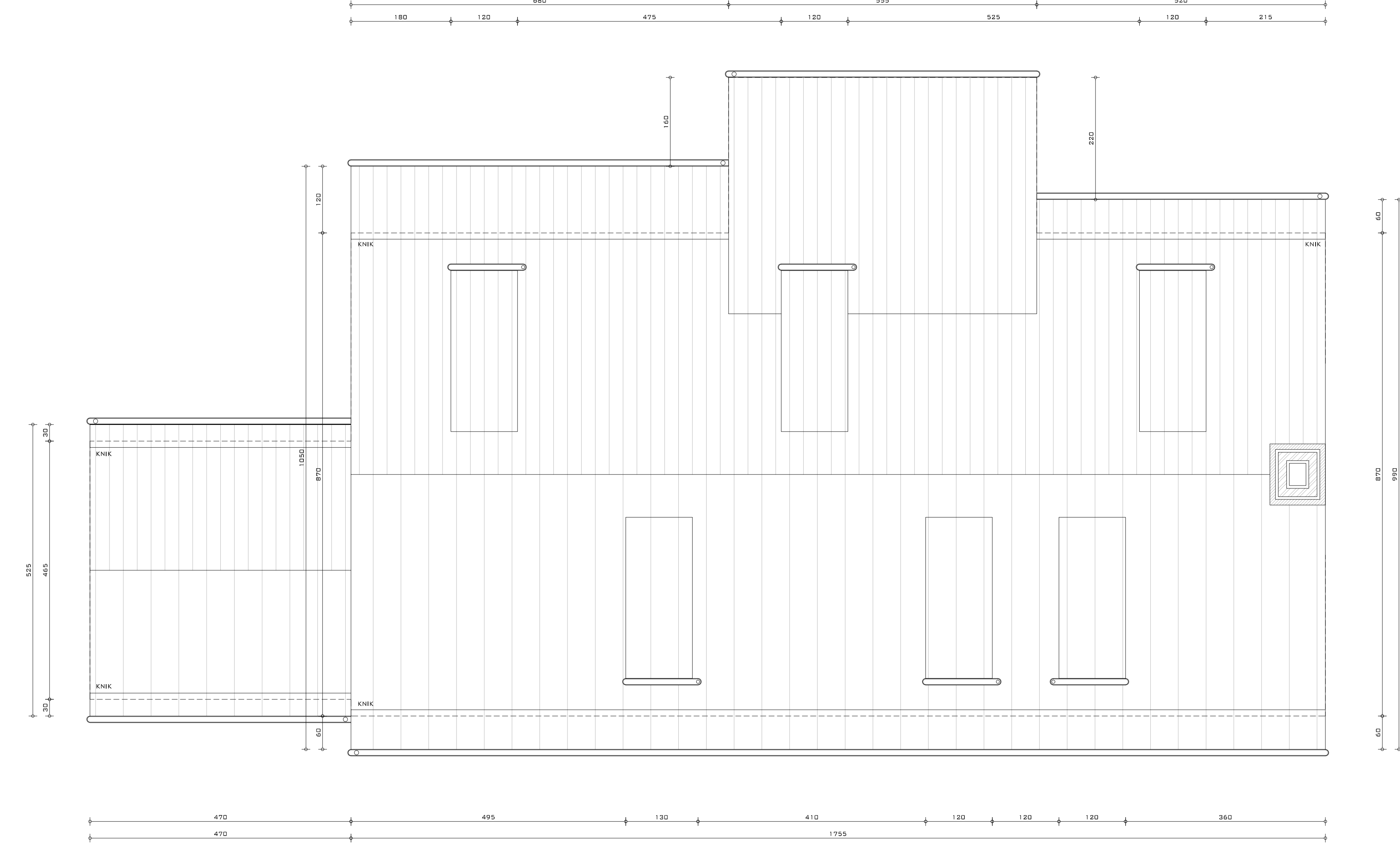
DAKENPLAN
