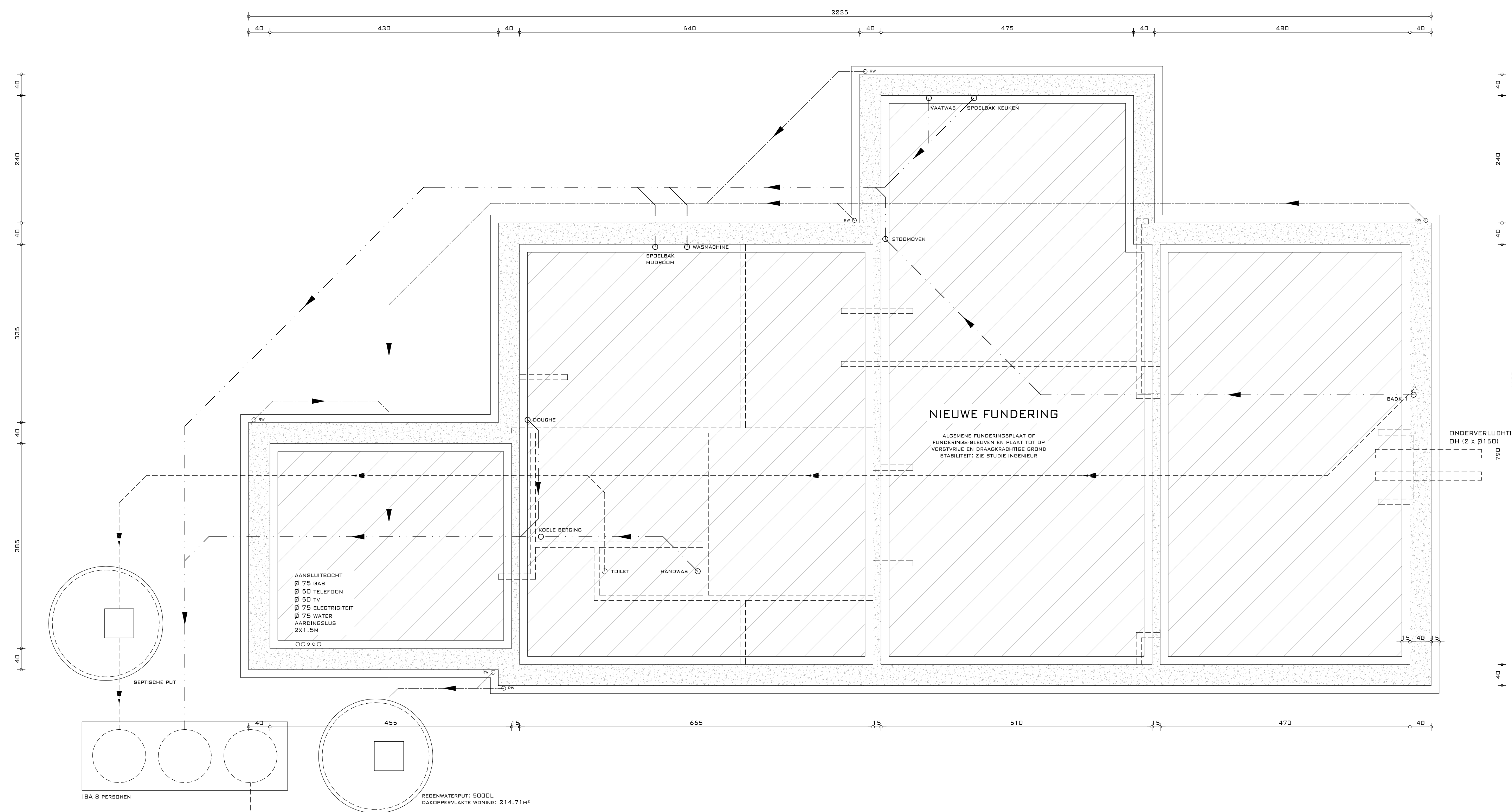
FUNDERING RIOLERING
